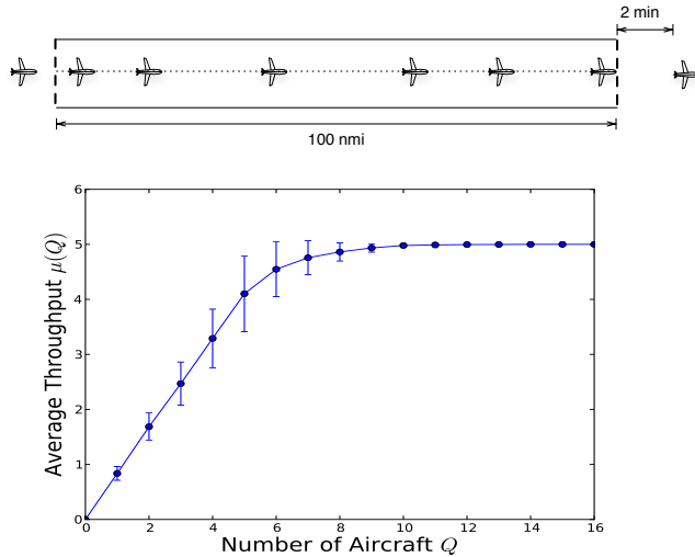
Fig. 2 Maximum throughput for the exit boundary of a simple linear control volume. The empirical curve of the mean number of departures per period was obtained via discrete-event simulation, with random arrivals. The error bars show the empirical variance of the number of departures per period. In this example, the exit boundary includes an explicit metering constraint, specifying a mandatory minimum separation of 2 min between successive aircraft.
