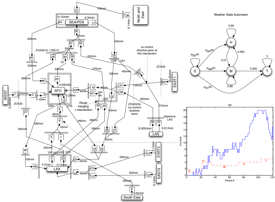
Fig. 9 Network model for TFM in the simulated system. Thick gray lines correspond to control variables coupled via the linear constraints (10), (11). All queues start initially empty. We also show the automaton describing the probabilistic weather evolution as well as a sample trajectory of a queue in the system under the MaxWeight policy. The red dashed line shows the evolution of the weather state for that sample, namely S - H - M - H - T .
