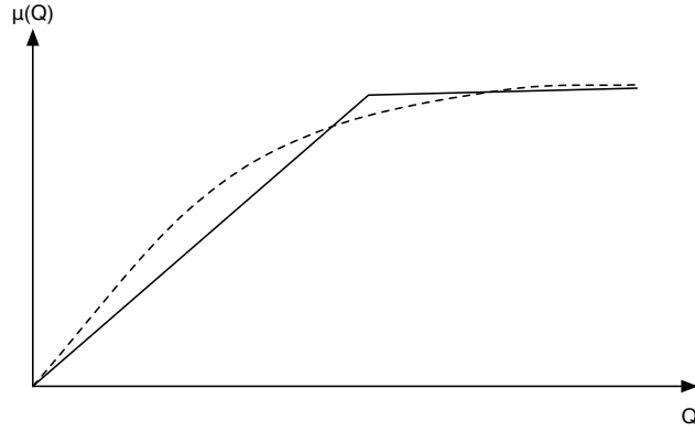
Fig. 4 Simple piecewise-linear approximation of the throughput curves used in the MPC optimization step, see (29).
