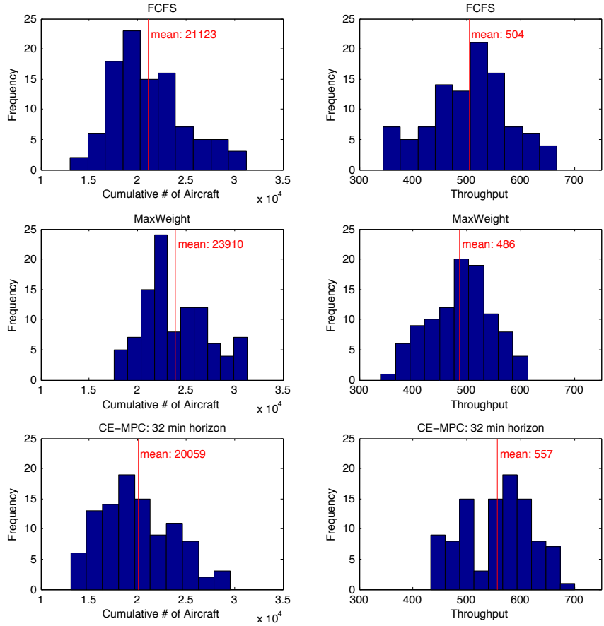
Fig. 10 Histograms of the performance results for 100 simulations, for a scenario with probabilistic forecasts as described on Fig. 9. Each simulation corresponds to an eight hour interval. On the left, we show the total cumulative number of aircraft in the system during the eight hour duration of the simulation. In other words, an aircraft is counted once for every period in which it remains in the system. On the right, we show the throughput of the policies, that is, the total number of aircraft that landed during the simulation.
