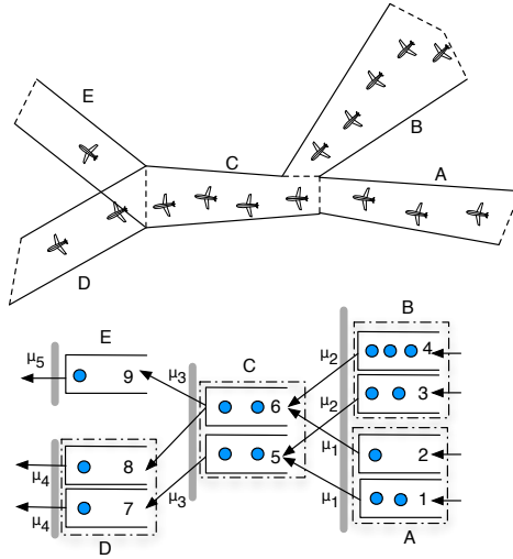
Fig. 1 Five control volumes and their corresponding abstract buffer model. The situation depicted here corresponds to two routes merging and then diverging. Each control volume except E supports two flows with distinct characteristics (e.g., different destinations, as described Section II B 1), and each flow is associated with one buffer. Buffers 8 and 9 have the same flow type (destination), which allows us to include routing decisions at the output boundary of volume C . Each buffer has an associated maximum throughput function, as discussed in Section II A. In this case, the buffers associated with the same control volume have the same maximum throughput function. Thick gray lines represent additional resource constraints coupling the control variables of different buffers, as described in Sections II B 1 and II B 2.
