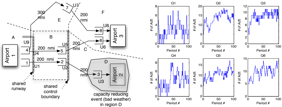
Fig. 5 Small scenario with geographic capacity constraints and a local bad weather event in region D . In the absence of bad weather (nominal conditions), the FCFS policy stabilizes the system, as shown on the right of the figure (100 periods of length T = 5 min each shown). Queues 1 – 6 start with 5 aircraft each.
