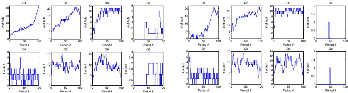
(a) Sample path for the MaxWeight policy with routing.
