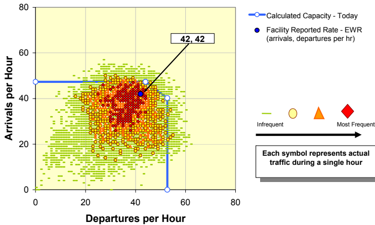
Fig. 3 Capacity envelope observed at Newark airport, under optimal conditions [27]. Any pair of arrival/departure allocation rates within the polytope is achievable. This polytope corresponds to constraints of the form (5), and depends on the airport runway configuration [28].
